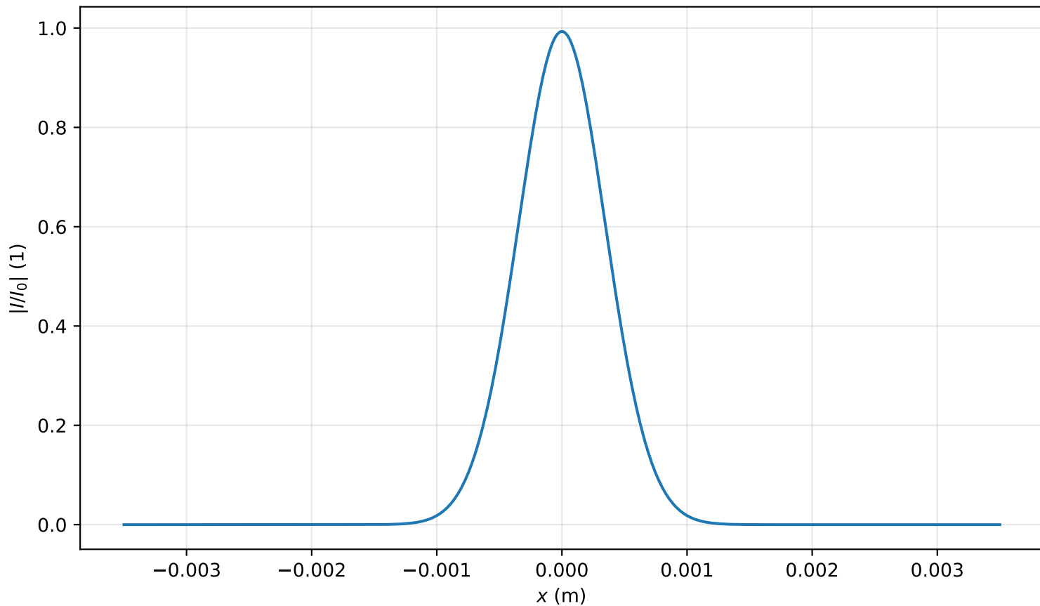
Intensity profile I(x, y = 0, z = 0.318m)/I_0 , P_{in}=0.2P_{cr} , artificial time
